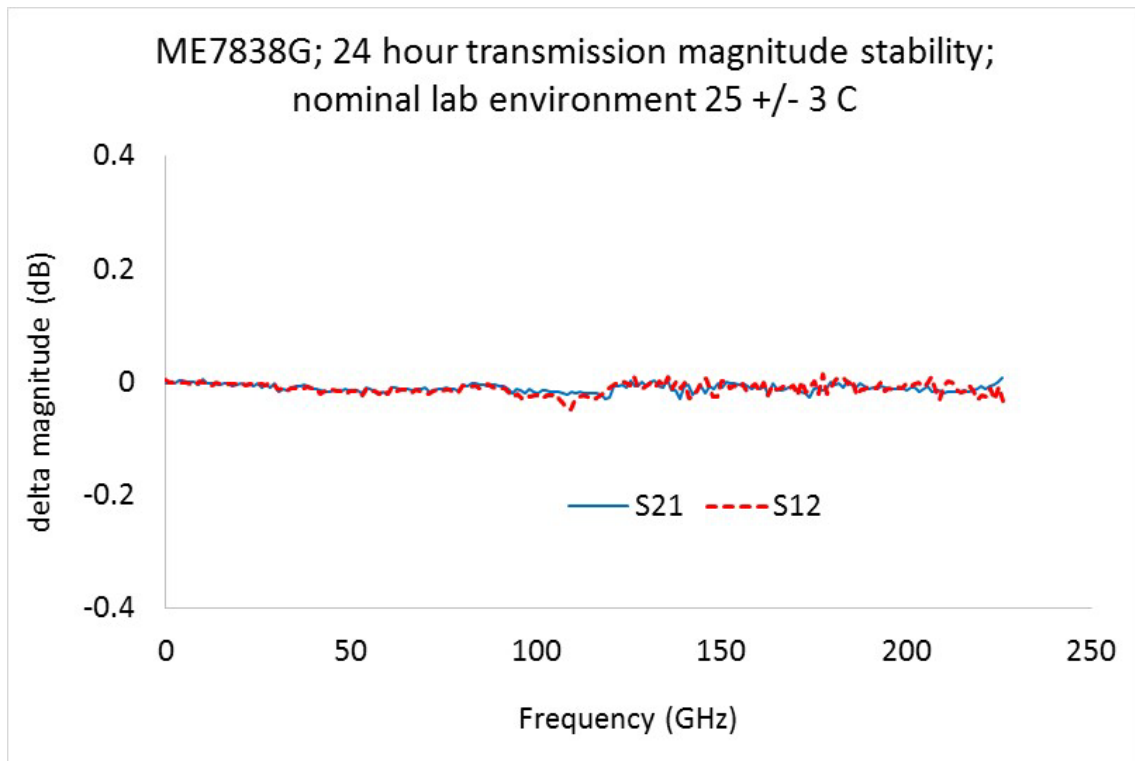
Example 24 Hour Transmission Magnitude Stability
