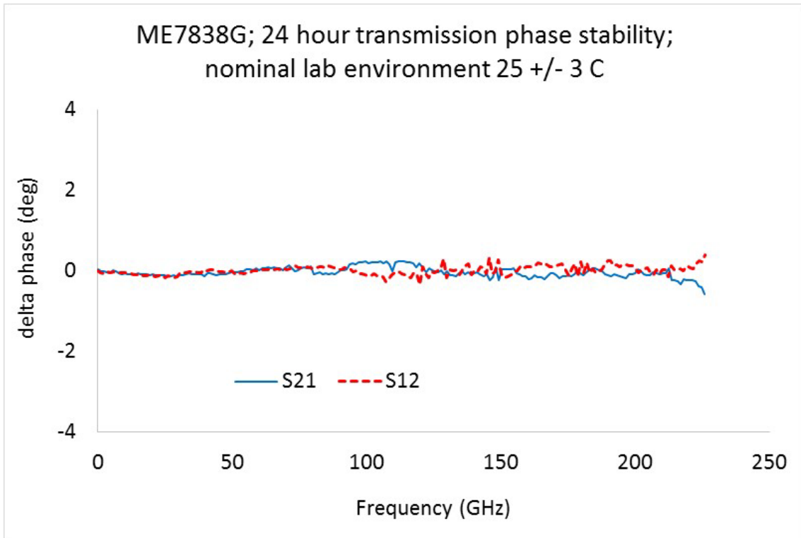
Example 24 Hour Transmission Phase Stability
