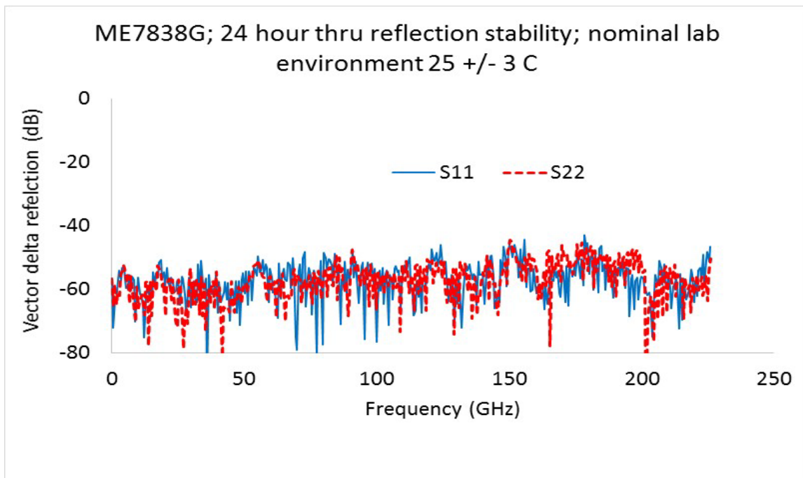
Example 24 Hour Thru Line Match Vector-delta Stability
