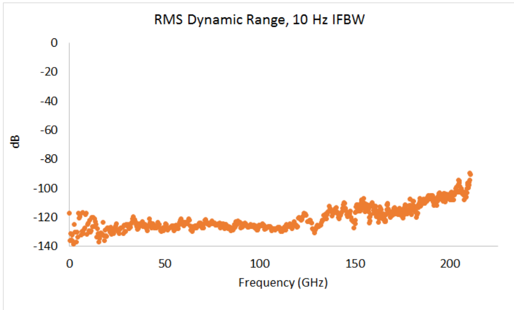
Example dynamic range of the ME7838G system at the flange interface connector from 70 kHz-220 GHz in a 10 Hz IF bandwidth. RMS computation.
